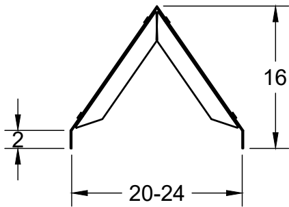
Adjustable Crossarm Fit
