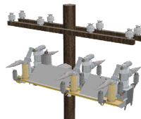
Intellirupter nest diverter kit
